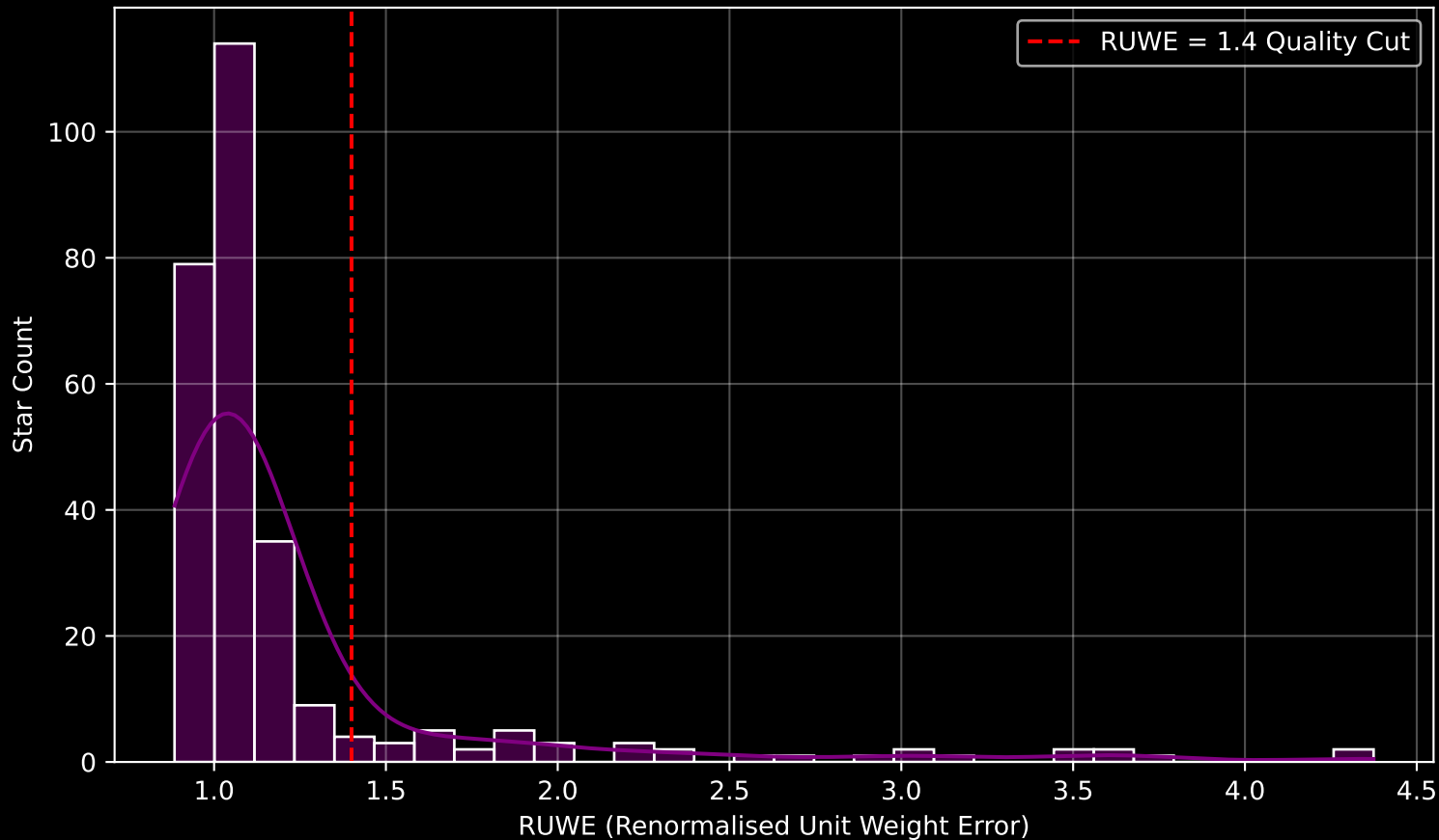
GALAH DR4 Field [269] RUWE Distribution (n= 277)
