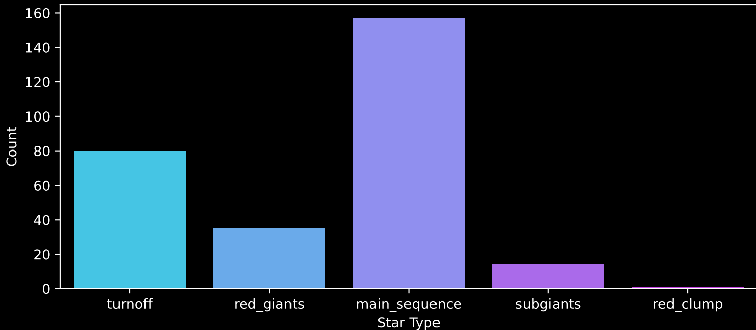
GALAH DR4 Field: [269] Count plot of Star Type
