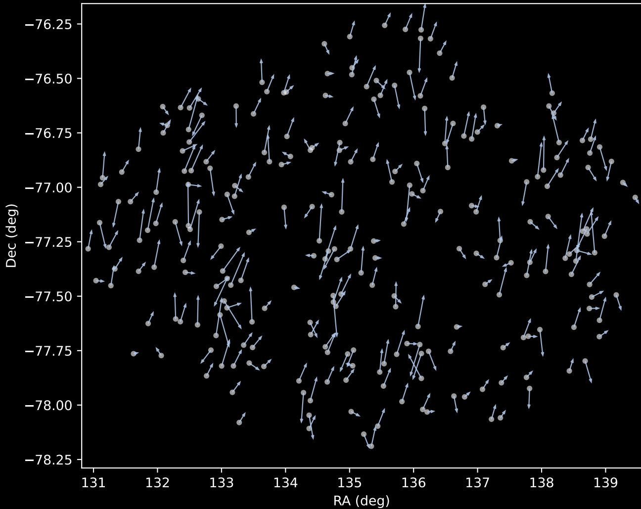
GALAH DR4 Cluster 1 Proper Motion Vectors (n=247)
